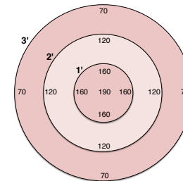
G8LED 90W Flower Booster Readings at 24"
