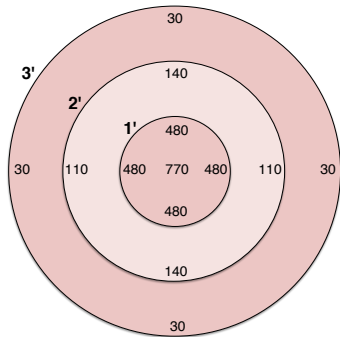
G8LED 90W Flower Booster Readings at 12"
