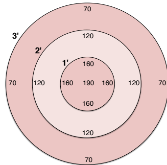
G8LED 90W Flower Booster Readings at 24"
