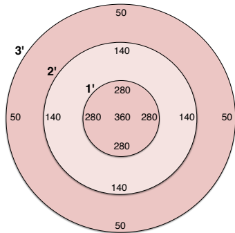
G8LED 90W Flower Booster Readings at 18"
